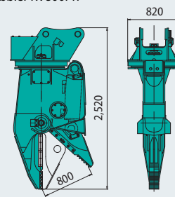
Car-dismantling nibbler KV800PR
